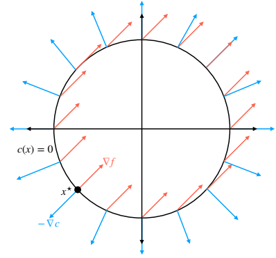
Figure 4: Illustration of the relationship between gradients of f and c .
