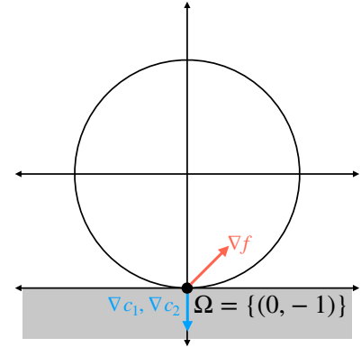
Figure 5: Illustration of objective and constraints in Example 22 .
