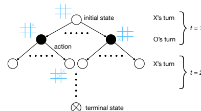
Figure 6: Extensive form of tic tac toe.
