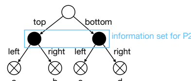
Figure 7: Extensive form for saddle point matrix game.
